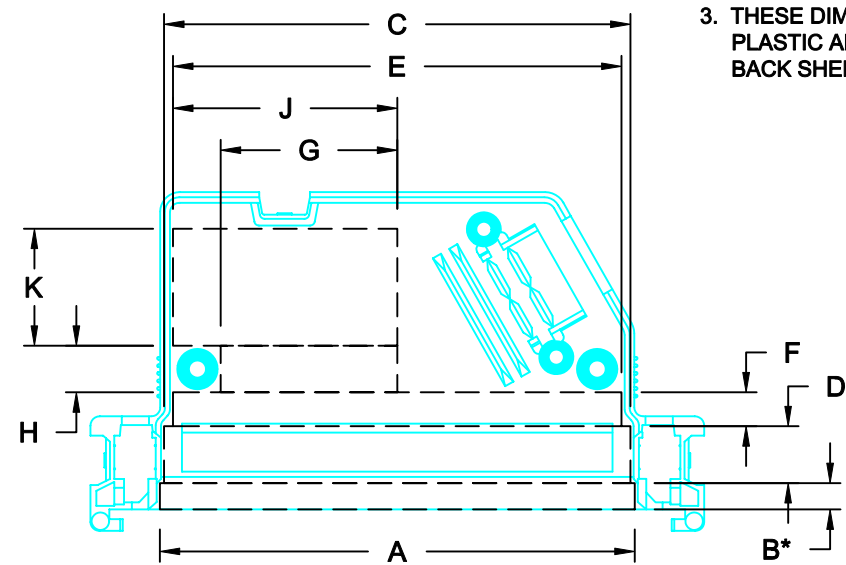
37-PIN
