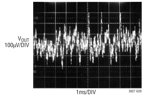
10Hz to 100kHz Output Noise C_{\text{BYP}} = 100\text{pF}
