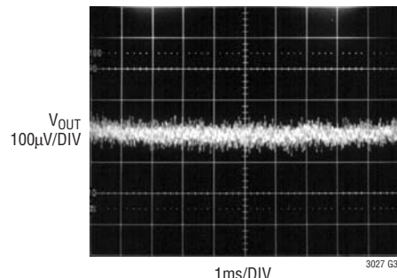
10Hz to 100kHz Output Noise C_{\text{BYP}} = 0.01\mu\text{F}
