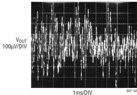
10Hz to 100kHz Output Noise C_{\text{BYP}} = 0
