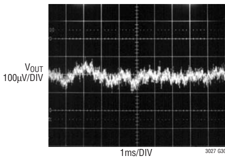
10Hz to 100kHz Output Noise C_{\text{BYP}} = 1000\text{pF}
